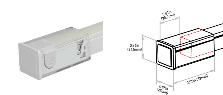
END CAP: 7-I-8
