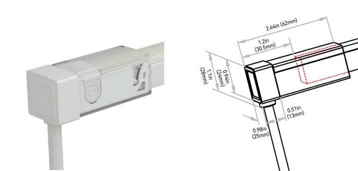
SIDE LEFT EXIT: 7-C-#
