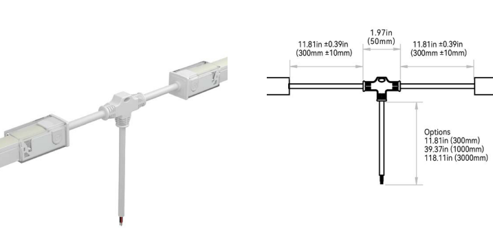
POWER T-FEED: 7-H-#
