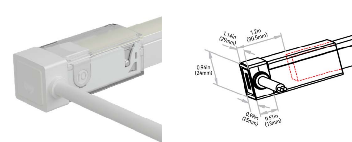
SIDE RIGHT EXIT: 7-D-#
