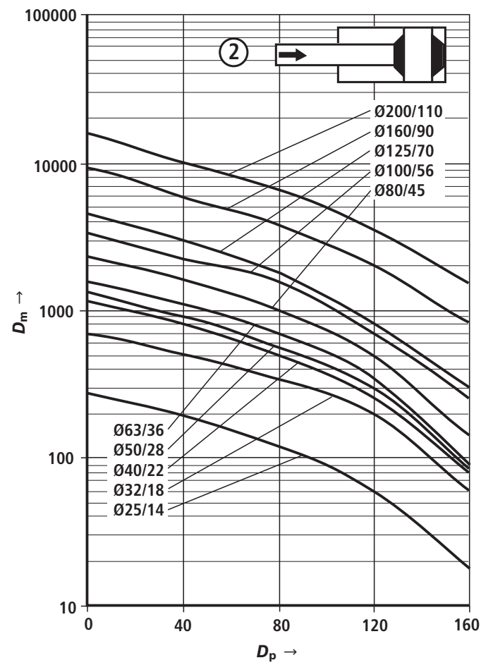
Damping capacity: Retraction and extension with k_v ②
