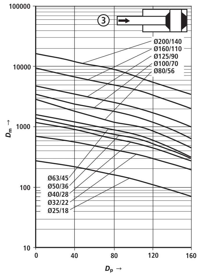
Damping capacity: Retraction and extension with k_v ③
