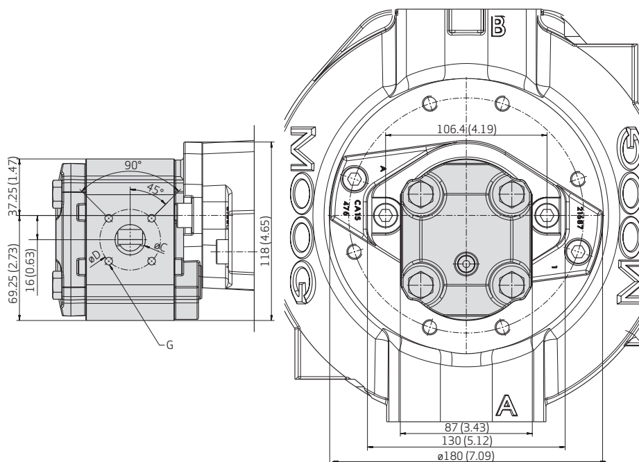
SAE-A Suction Side, Side View
