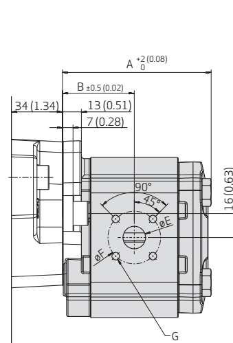
SAE-A Pressure Side, Side View
