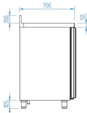
RIGHT VIEW
