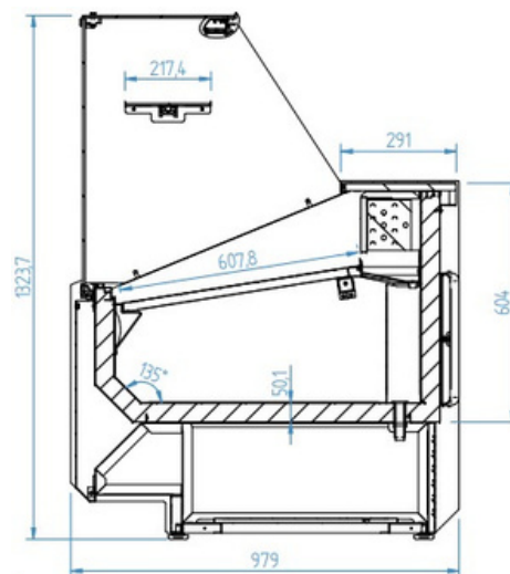
RIGHT VIEW
