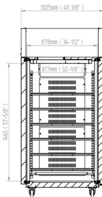
RIGHT VIEW
