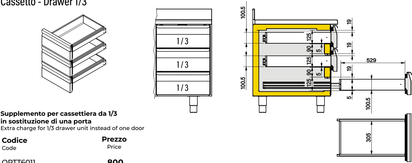
Cassetto - Drawer 1/3
