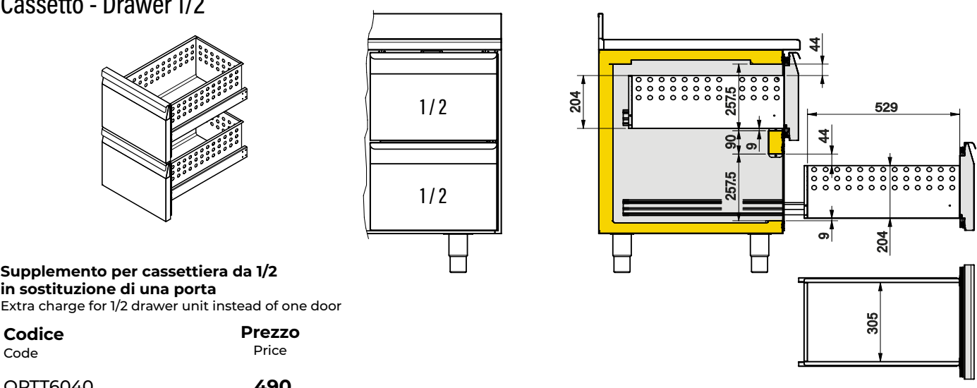
Cassetto - Drawer 1/2
