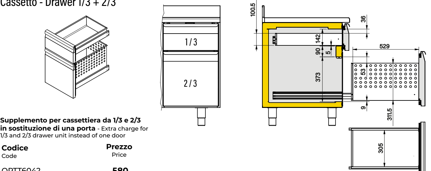
Cassetto - Drawer 1/3 + 2/3
