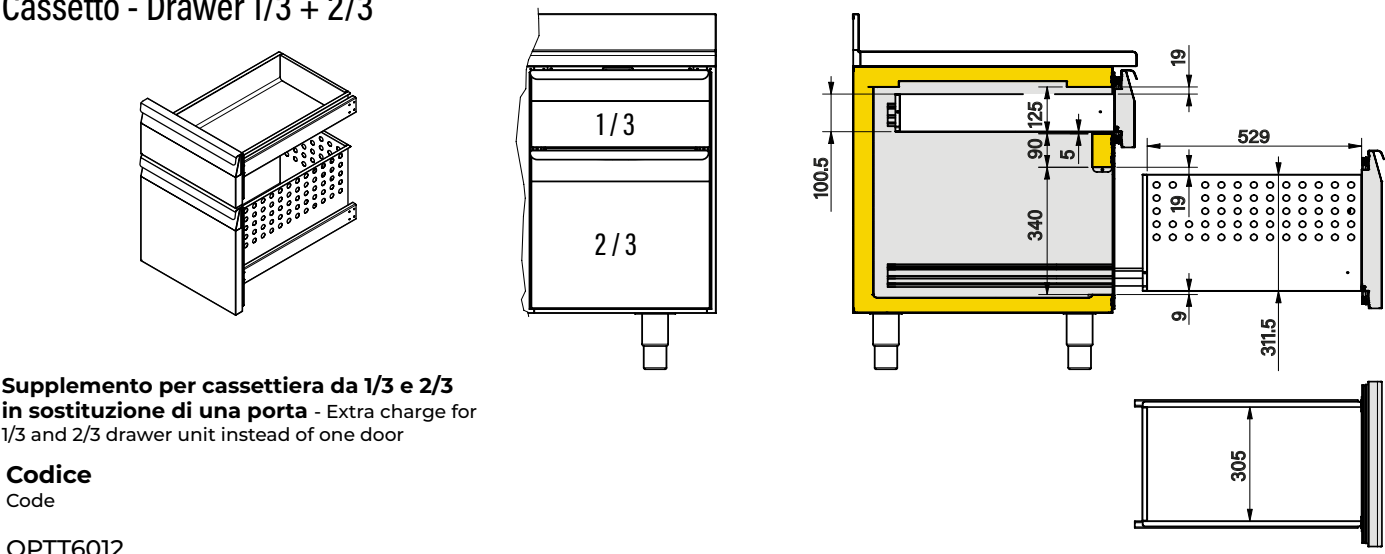
Cassetto - Drawer 1/3 + 2/3
