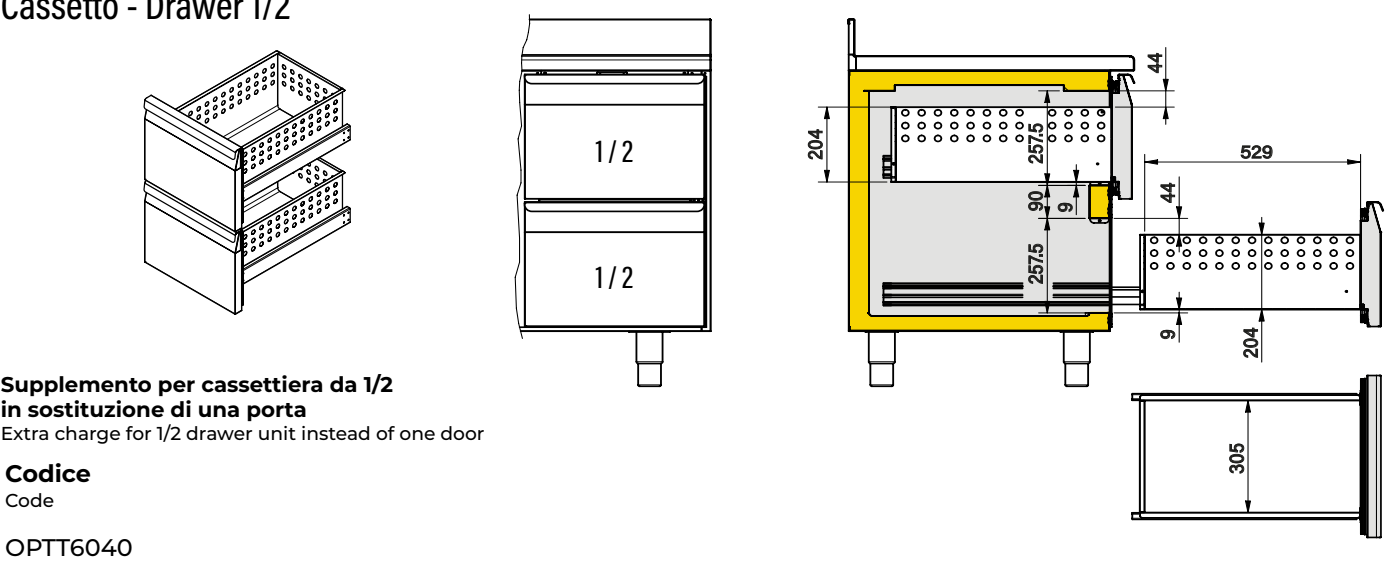
Cassetto - Drawer 1/2
