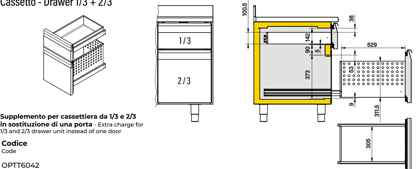
Cassetto - Drawer 1/3 + 2/3
