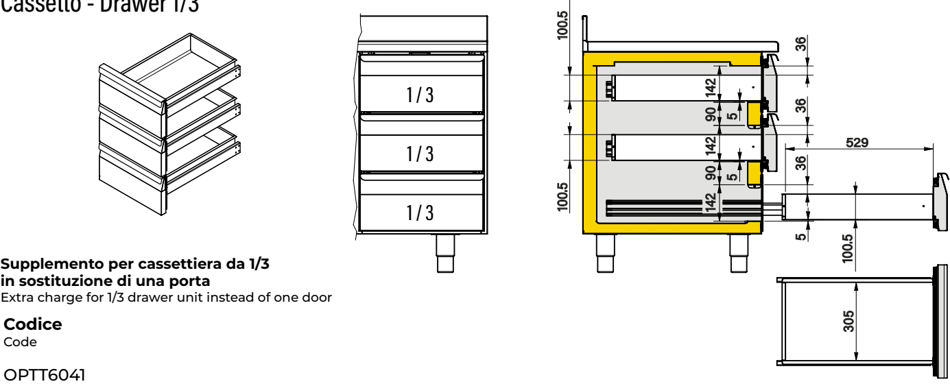
Cassetto - Drawer 1/3
