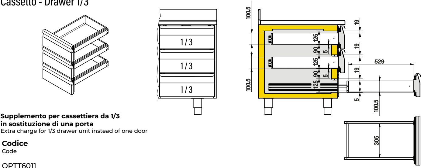
Cassetto - Drawer 1/3
