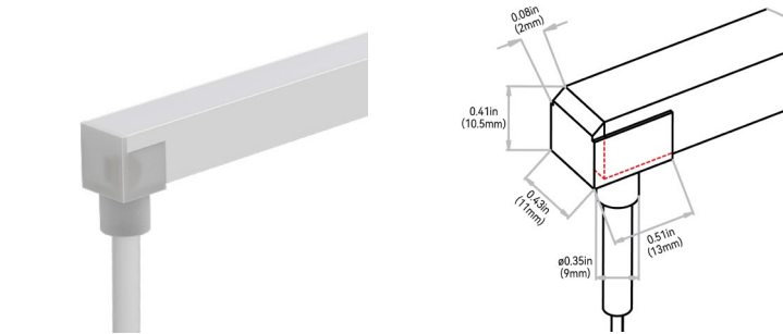
SIDE LEFT EXIT: E##2C#
