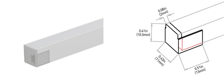
END JUMPER: E##2E1
