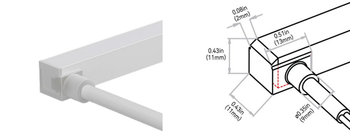
SIDE RIGHT EXIT: E##2D#
