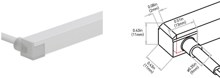
SIDE RIGHT EXIT: E##2D#
