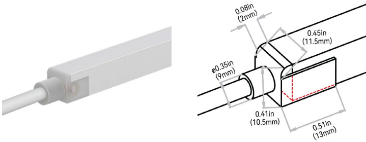
BOTTOM EXIT: E##2B#
