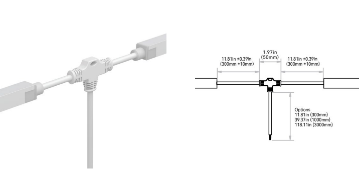
POWER T-FEED: K##2H#
