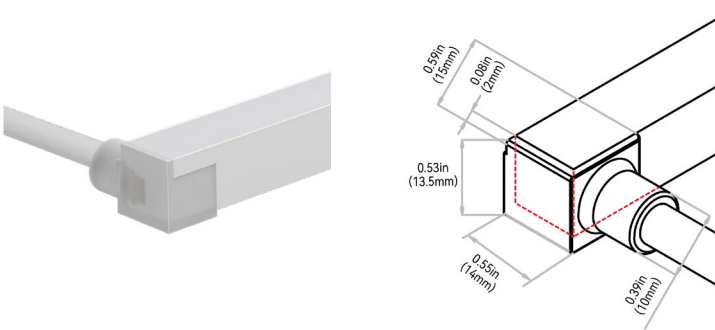
SIDE RIGHT EXIT: K##2D#
