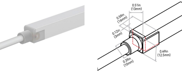
BOTTOM EXIT: K##2B#
