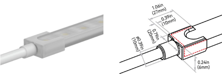
END EXIT: J2#2A#
