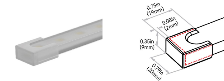
END JUMPER: J2#2E1
