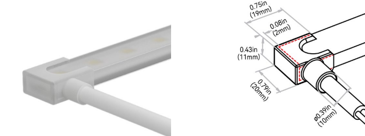
SIDE RIGHT EXIT: J2#2D#
