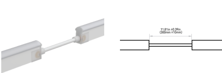
END JUMPER: C152E1
