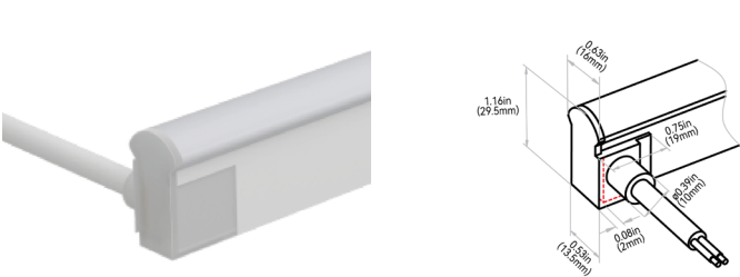
SIDE LEFT EXIT: C152C#
