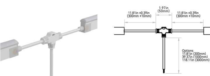
POWER T-FEED: C152H#
