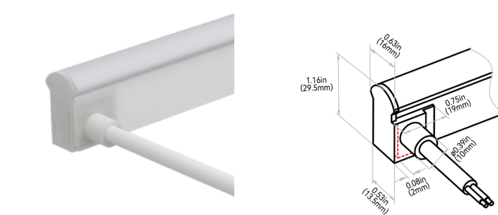
SIDE RIGHT EXIT: C152D#
