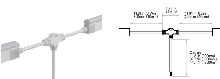
POWER T-FEED: C112H#
