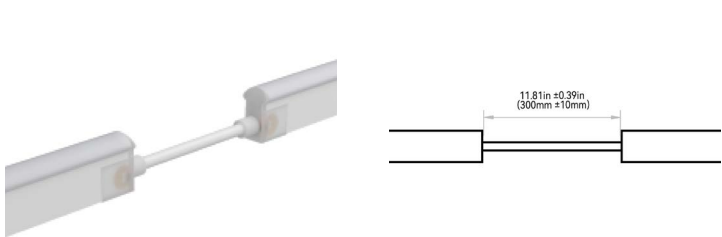
END JUMPER: C112E1
