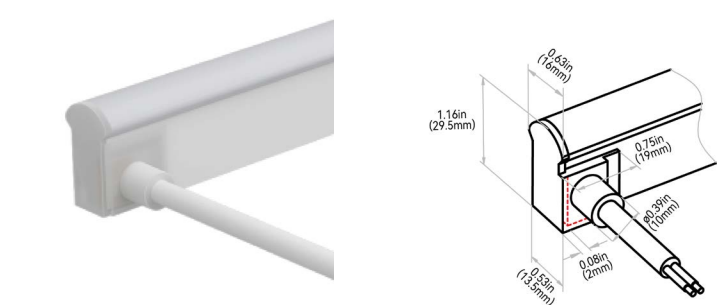
SIDE RIGHT EXIT: C142D#
