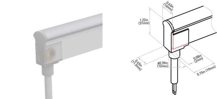
SIDE LEFT EXIT: C142C#
