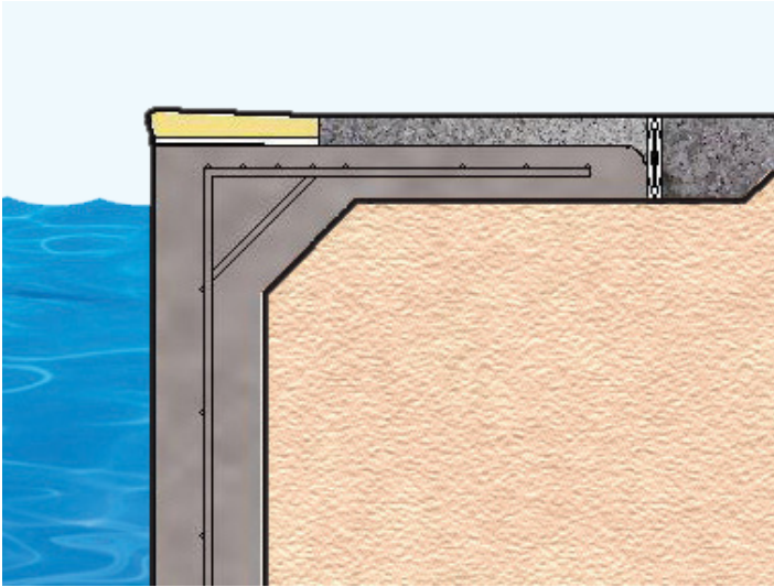
Gary Pools Cantilever
