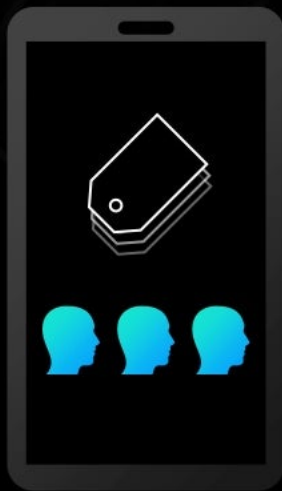
Crowdsources Labeling
