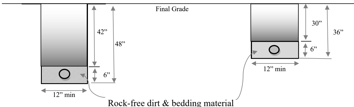
Primary Trench
