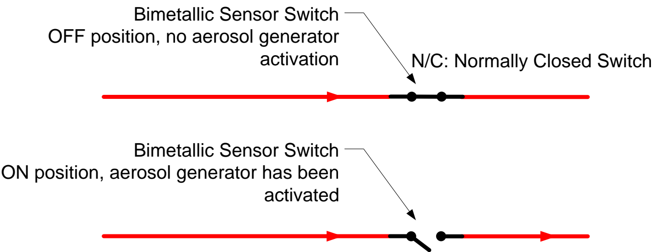
Bimetallic sensor
