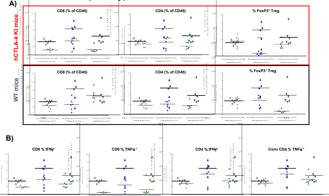
Figure 4. MC38 tumors from CTLA-4-KI humanized treated with ipilimumab or murine anti-CTLA-4 (days 5,8,11) were harvested 24 post last dose for immunophenotyping via Flow Cytometry. A) Percentage of T regs, CD4 and CD8 T cells present in the tumor tissue of CTLA-4-KI or WT mice. B) T cell ex-vivo stimulation shows increase levels of IFN \gamma and TNF \alpha in both CD4 and CD8 T cells of CTLA-4-KI humanized treated mice
