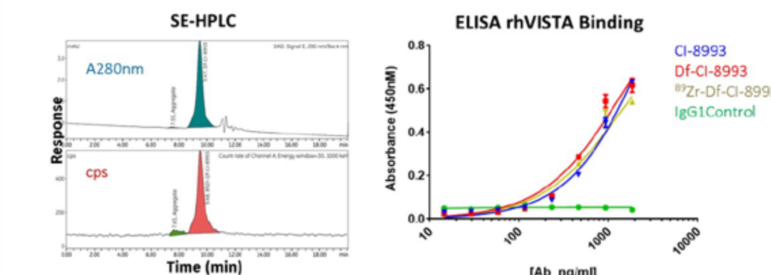
Figure 3. Left: Size exclusion (SE) HPLC A280 and counts per second (CPS) scintillation trace of 89 Zr-Df-CI-8993. Right: ELISA analysis binding recombinant human VISTA (R&D Systems).
