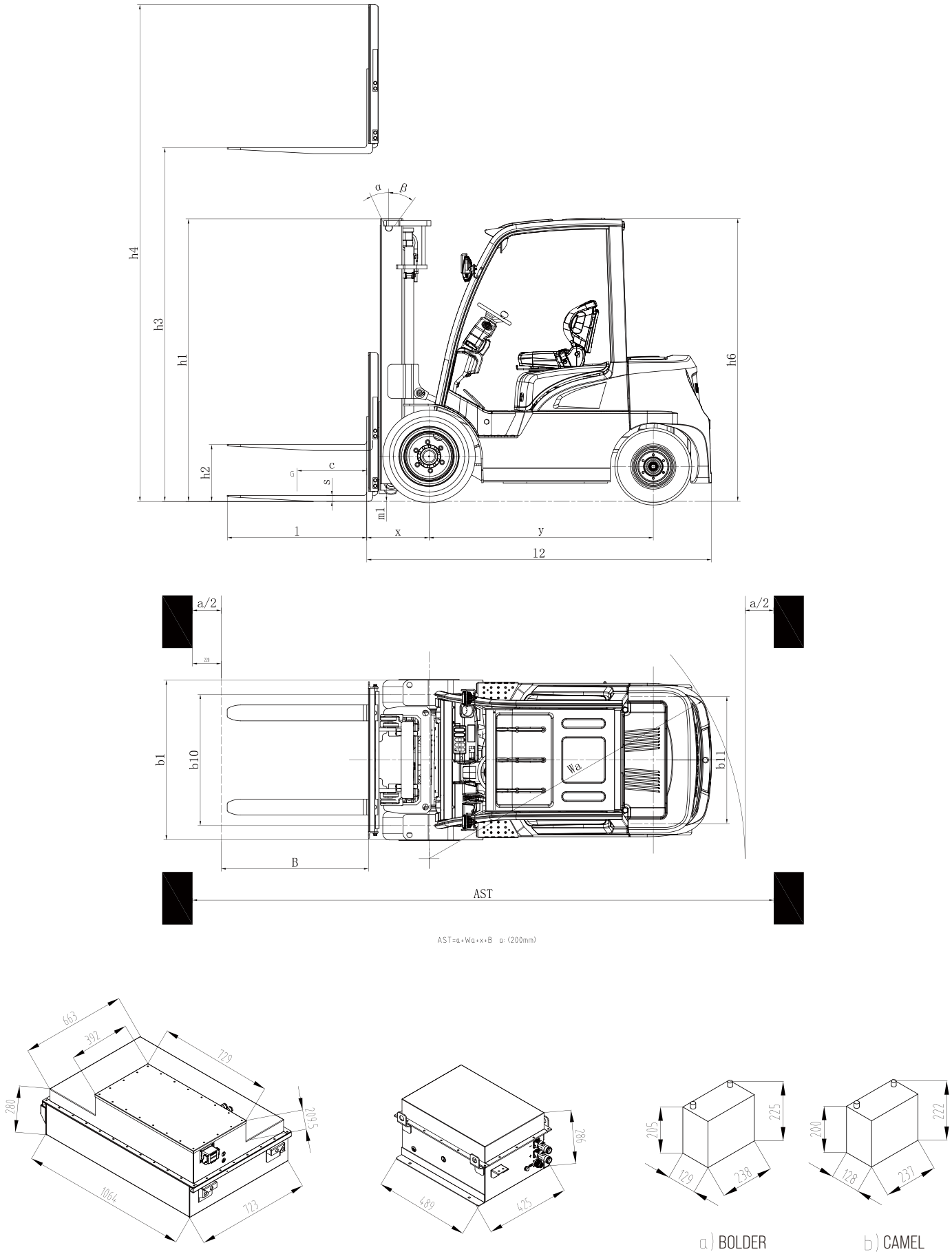
Dimension of lithium battery main box
