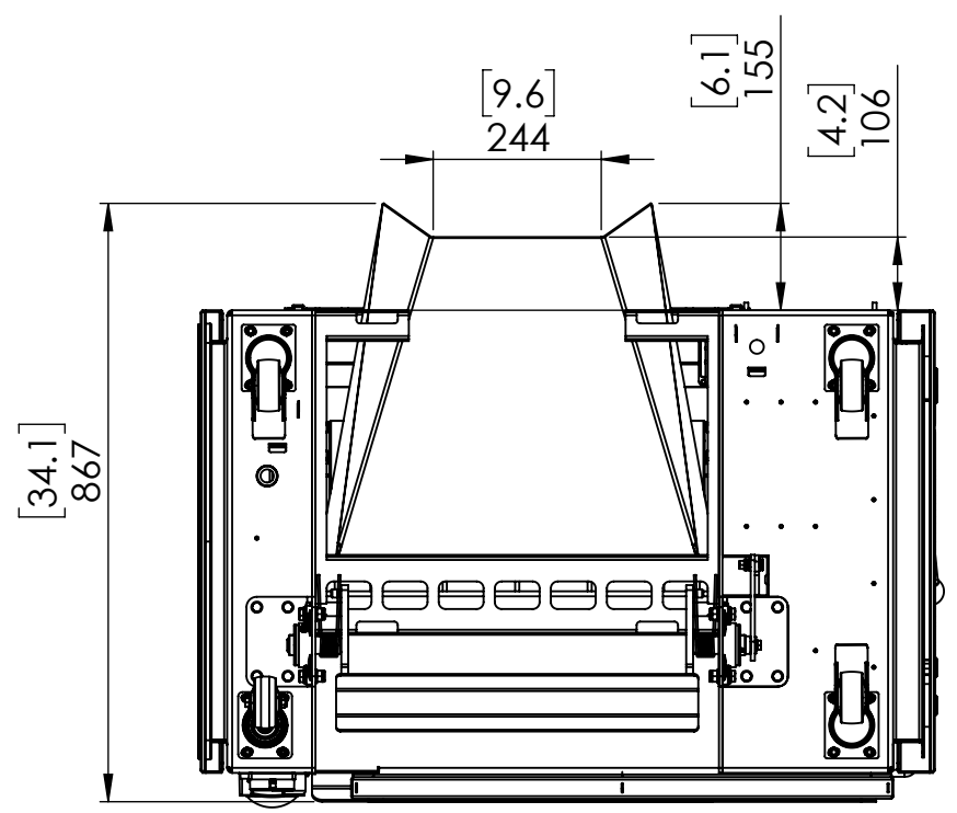
BACK CHUTE CONFIGURATION
