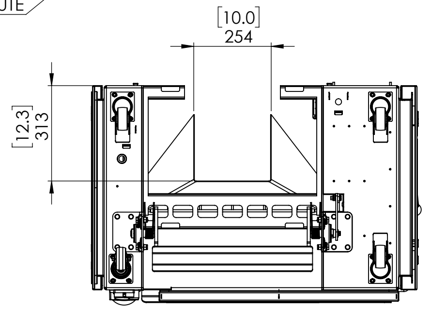
BOTTOM CHUTE CONFIGURATION
