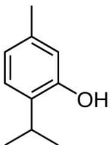
Thymol
