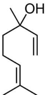
Linalol
