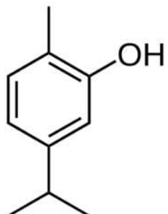
Carvacrol
