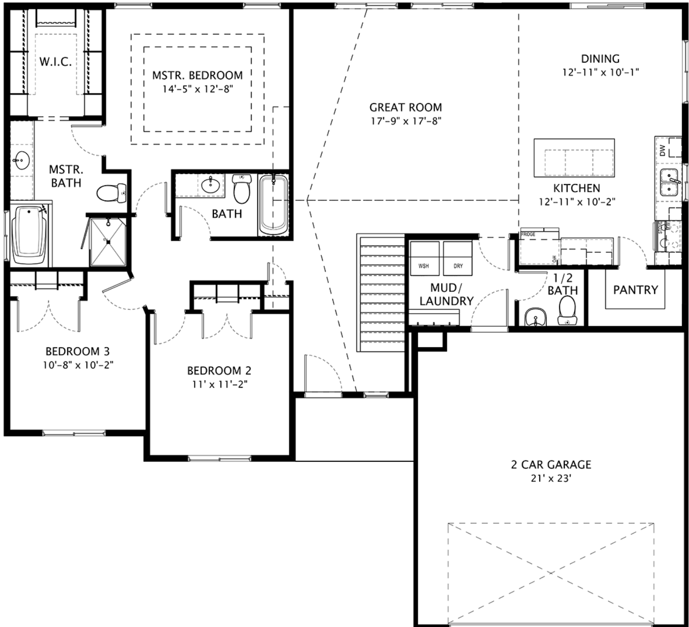
Main Floor
