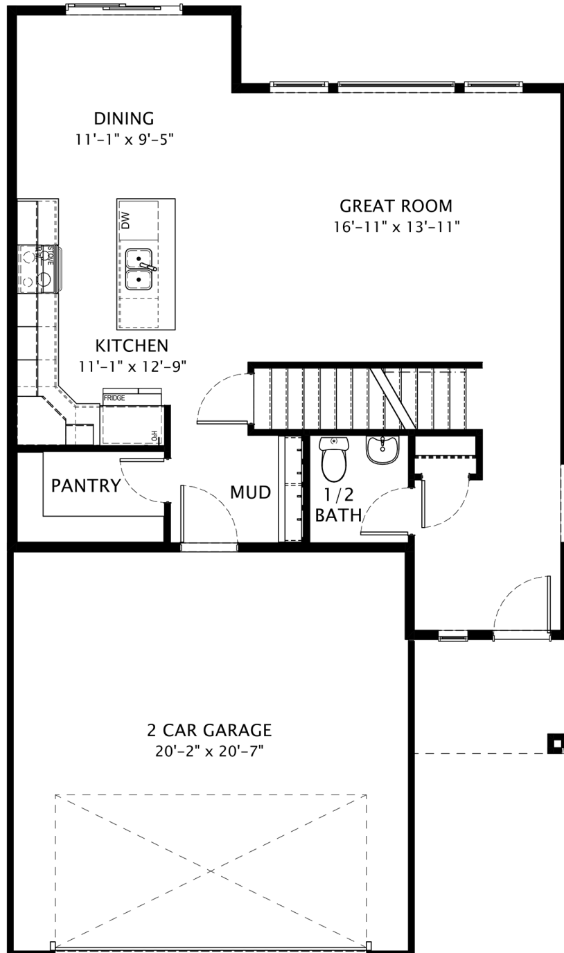
Main Floor
