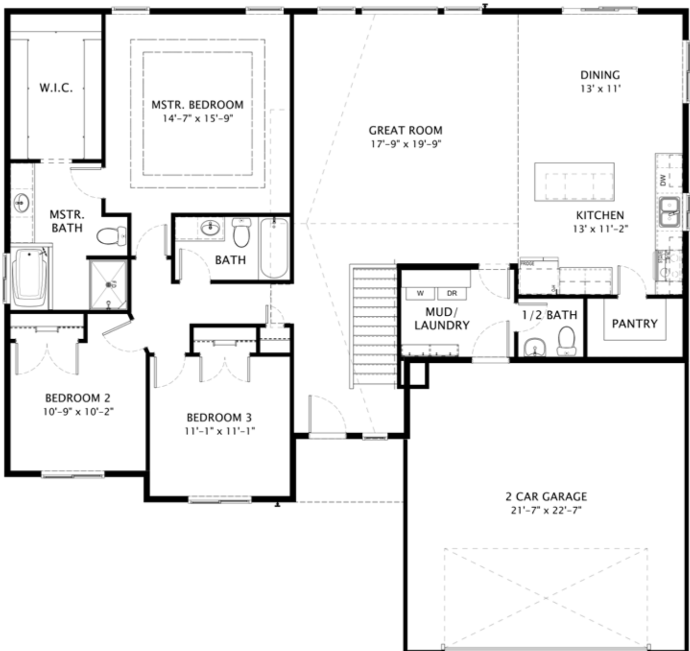
Main Floor
