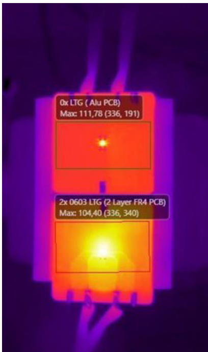
Picture 1: (Upper) Alu with LTG (0603*0) at 111.78°C. (Bottom) 2-layer FR4 with LTG (0603*2) at 104.40°C.
