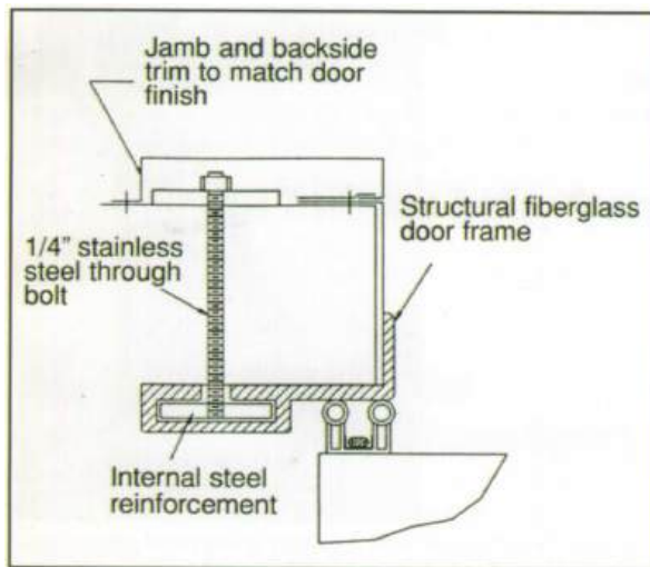
Single Horizontal Sliding Diagram
