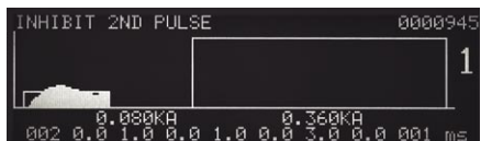
Run screen – shows that second pulse was inhibited from firing.
