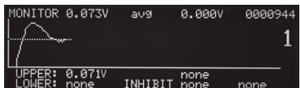
Monitor screen – shows first pulse weld voltage exceeded limit.
