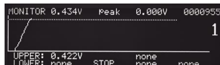
Monitor screen – shows weld voltage exceeding limit.
