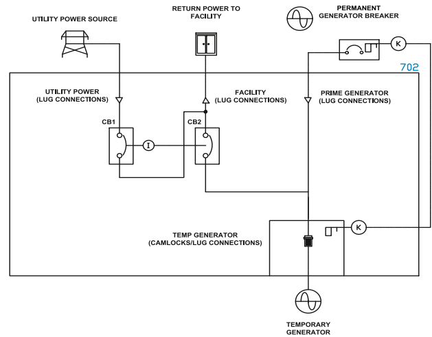
DUAL BREAKER ATS DOCKING STATION - SERVICE ENTRANCE RATED ATS WITH TEMPORARY GENERATOR CONNECTION. TEMPORARY GENERATOR CAMPLATE KIRK KEY INTERLOCKED UPSTREAM CLIENT PERMANENT GENERATOR BREAKER.
