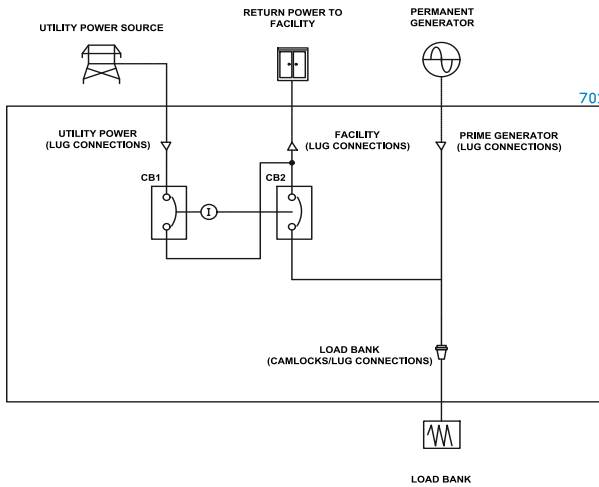
DUAL BREAKER ATS DOCKING STATION - SERVICE ENTRANCE RATED ATS WITH LOAD BANK TESTING.
