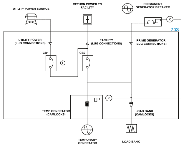
DUAL BREAKER ATS DOCKING STATION - SERVICE ENTRANCE RATED ATS WITH TEMPORARY GENERATOR CONNECTION AND LOAD BANK TESTING. TEMPORARY GENERATOR CAMPLATE KIRK KEY INTERLOCKED UPSTREAM CLIENT PERMANENT GENERATOR BREAKER.
