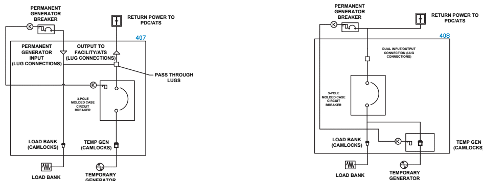
SINGLE BREAKER DOCKING STATION - SYSTEM BREAKER IS INTERLOCKED WITH UPSTREAM GENERATOR BREAKER VIA KIRK KEY. INCLUDES DUAL PURPOSE PASS THROUGH LUGS
