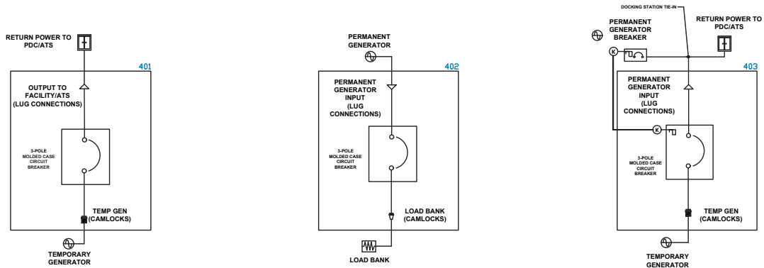
SINGLE BREAKER DOCKING STATION TEMPORARY GENERATOR CONFIGURATION
