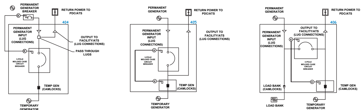
SINGLE BREAKER DOCKING STATION - SYSTEM BREAKER IS INTERLOCKED WITH UPSTREAM GENERATOR BREAKER VIA KIRK KEY. INCLUDES PASS THROUGH LUGS
