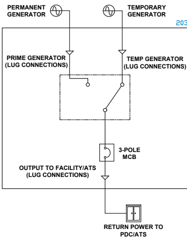
ROTARY MANUAL TRANSFER SWITCH WITH DISCONNECTING MEANS ON OUTPUT
