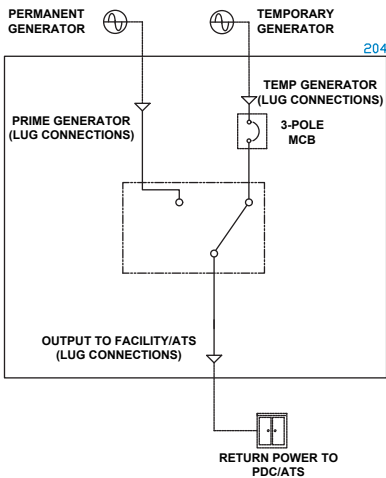
ROTARY MANUAL TRANSFER SWITCH WITH DISCONNECTING MEANS ON TEMPORARY GENERATOR INPUT
