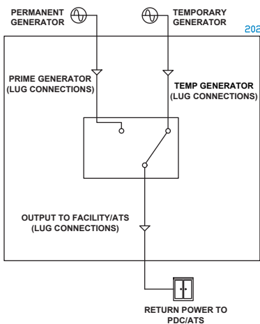
ROTARY MANUAL TRANSFER SWITCH
