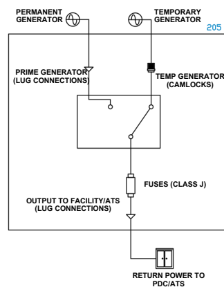
FUSED ROTARY MANUAL TRANSFER SWITCH
