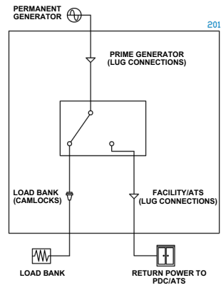
ROTARY MANUAL TRANSFER SWITCH CONFIG 1
