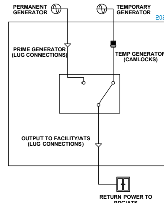
ROTARY MANUAL TRANSFER SWITCH CONFIG 2
