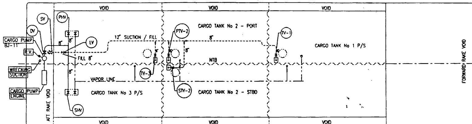
CARGO PIPING
