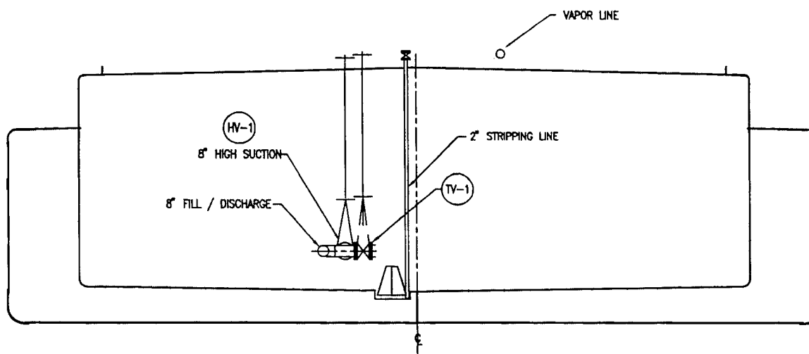
BELOW DECK PIPING
