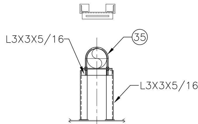
DETAIL "8" 8" PIPE SUPPORT
