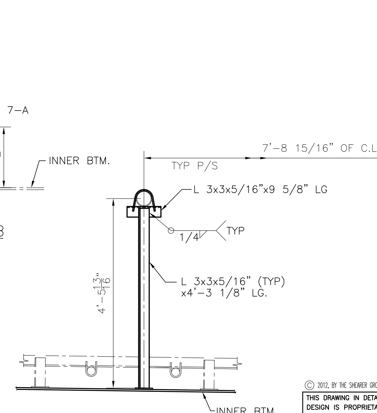
DETAIL 3-A 3/4" = 1'-0"
