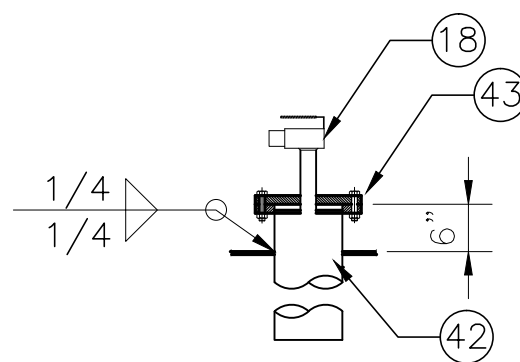
DETAIL "2" HIGH LEVEL/ALARM SHUTDOWN
