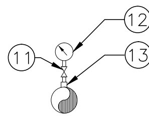
DETAIL "7" PUMP DISCHARGE PRESSURE GAUGE NTS
