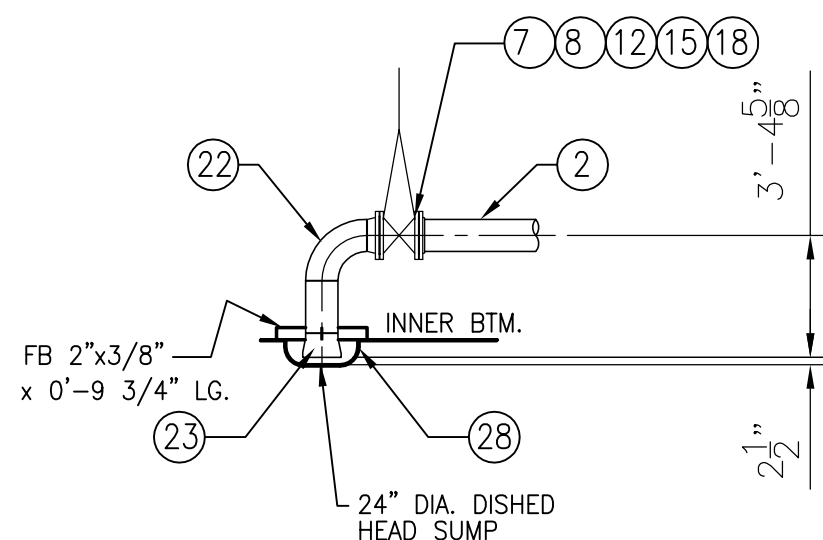
SECTION H-H SCALE:- 3/16"=1'-0"
