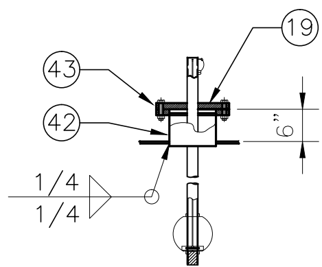
DETAIL "1" HIGH LEVEL INDICATOR 1/2" = 1'-0"
