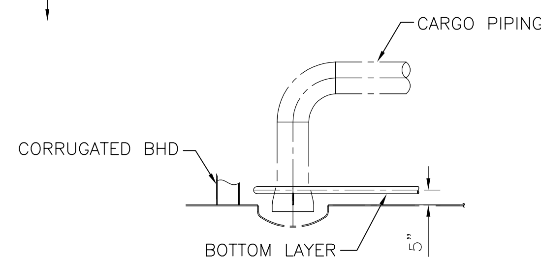
SECTION 5-A 3/8" = 1'-0"
