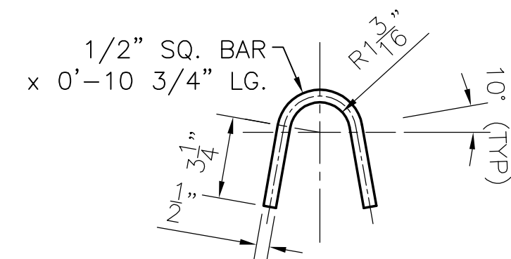
DETAIL 7-A 2 1/4" = 1'-0"
