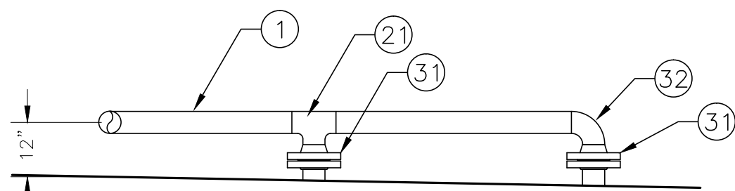
DETAIL "4" VAPOR CONNECTION
