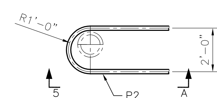
DETAIL 4-A 3/8" = 1'-0"
