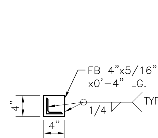
DETAIL 8-A 1 1/8" = 1'-0"
