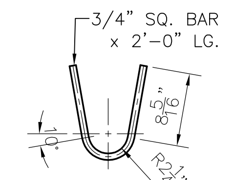
DETAIL 1-A 1 1/8" = 1'-0"
