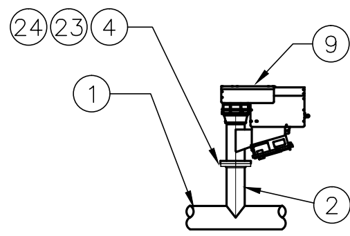
DETAIL "3" P-V VALVE
