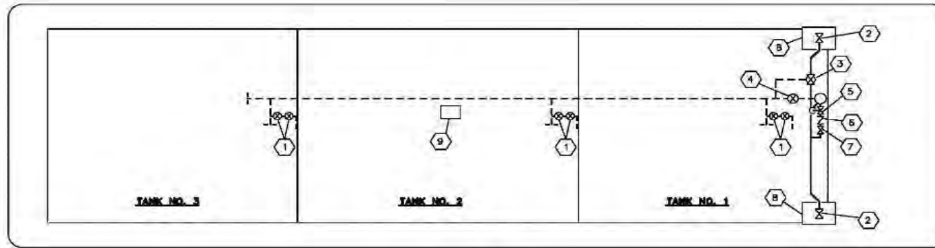
CARGO PIPING
