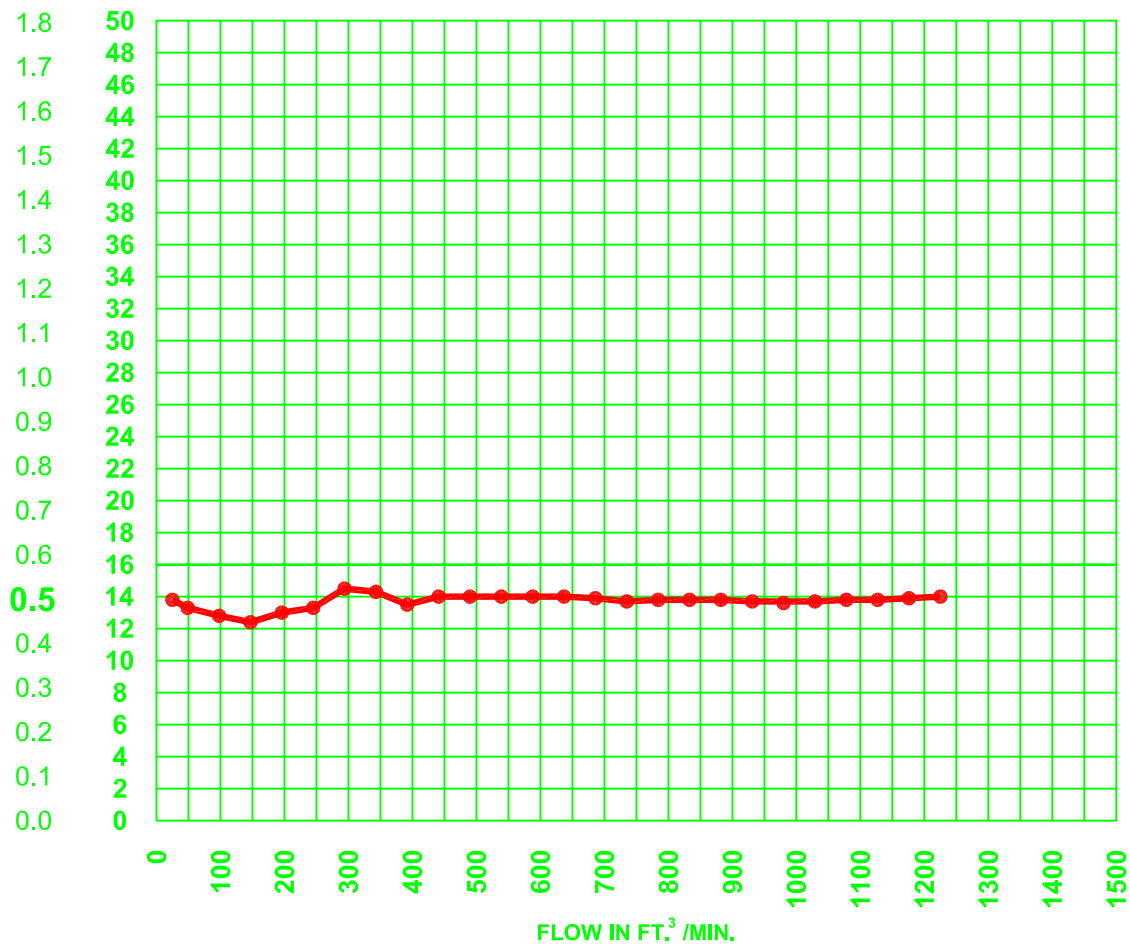
CURVE FOR VACUUM SIDE OF 6" PV VALVE - 0.5 PSI DATA BASED ON AIR FLOW
