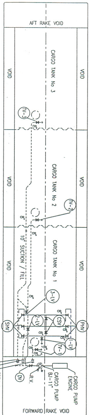
CARGO PIPING
