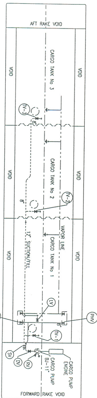
CARGO PIPING
