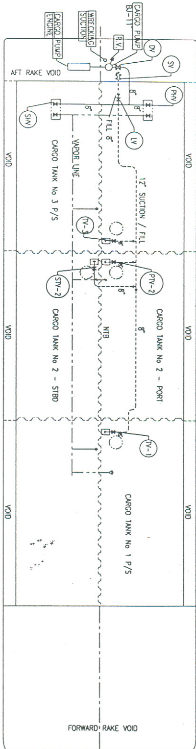
CARGO PIPING
