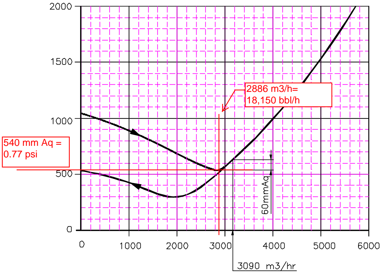
FLOW CAPACITY CURVE, SCM(HStandard cubic meter per hour) (1SCMH = 6.289BBL/hr)
