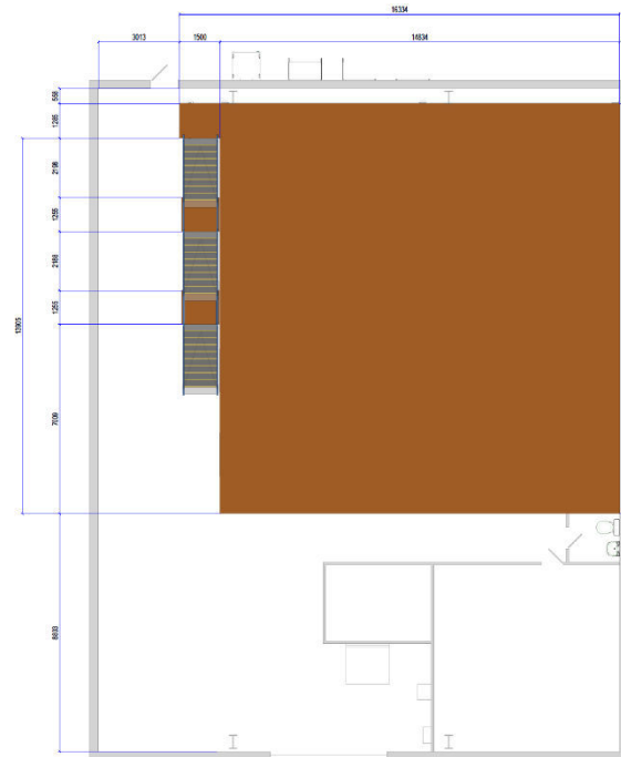
FLOOR DIMENSIONS
