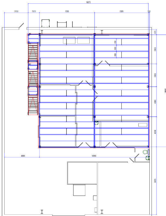
STEEL CONSTRUCTION
