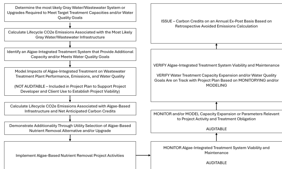
Figure 1: Methodology Overview
