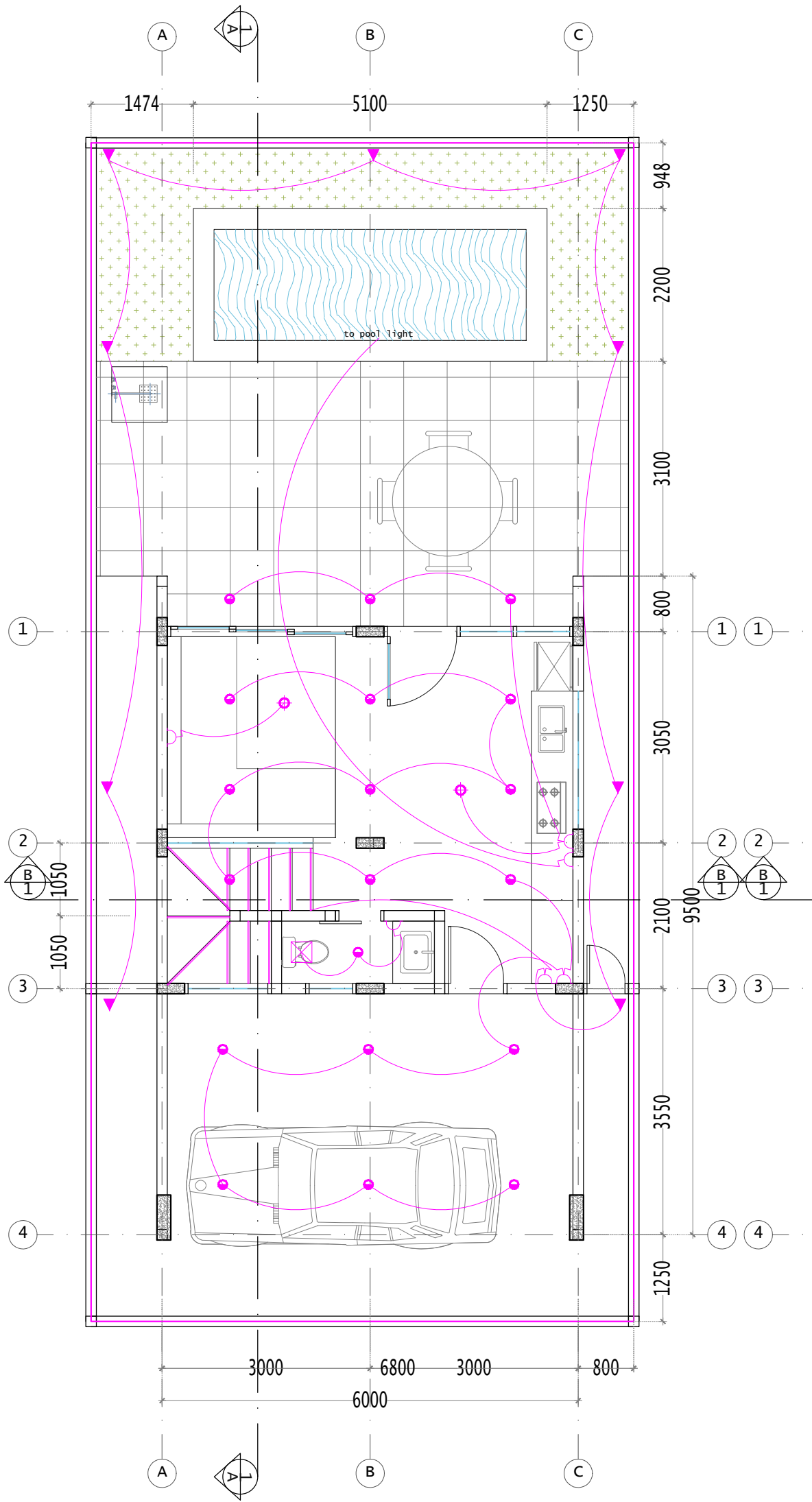
GROUND FLOOR LIGHTING PLAN | SCALE 1 : 75
