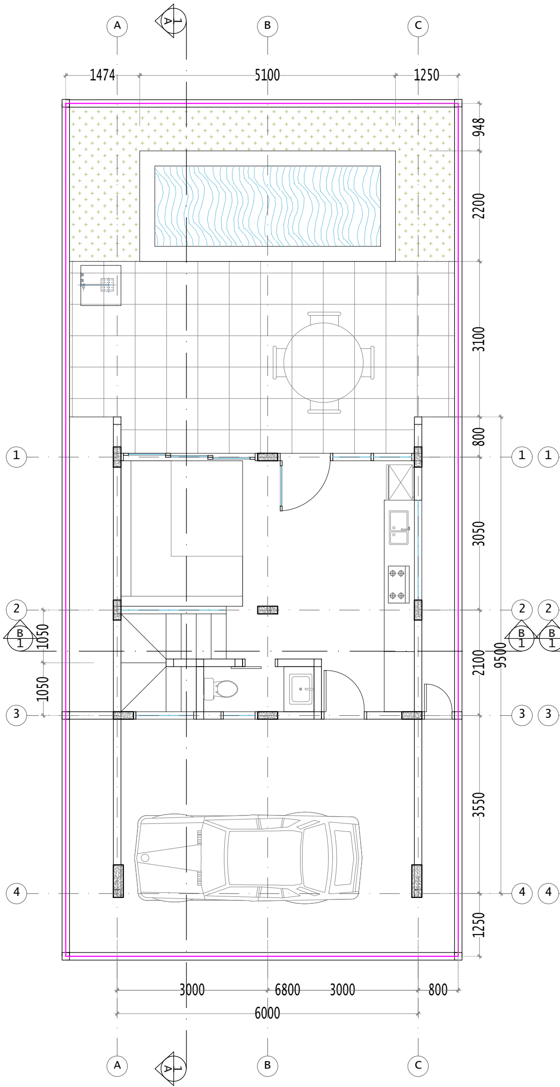
GROUND FLOOR SCALE 1 : 75
