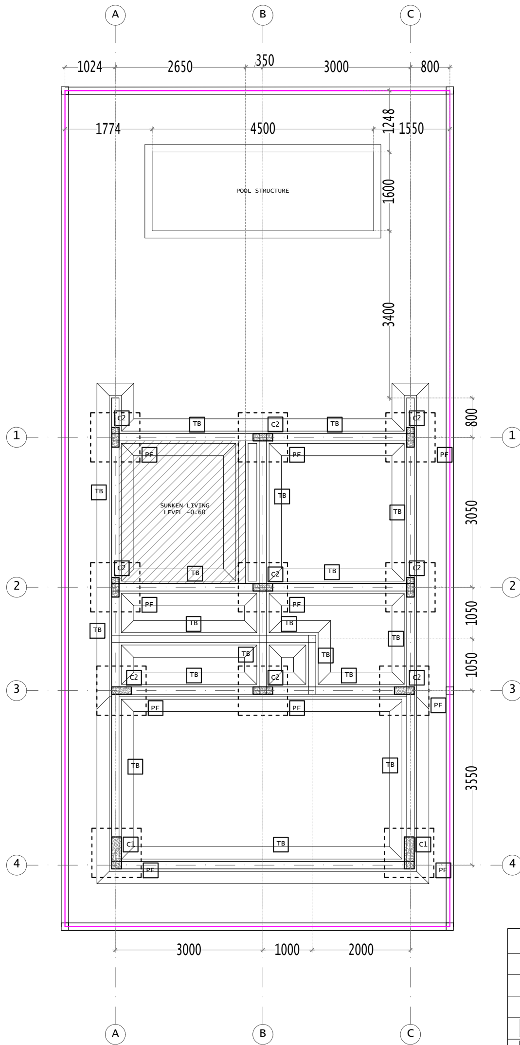
FOUNDATION PLAN SCALE 1 : 75
