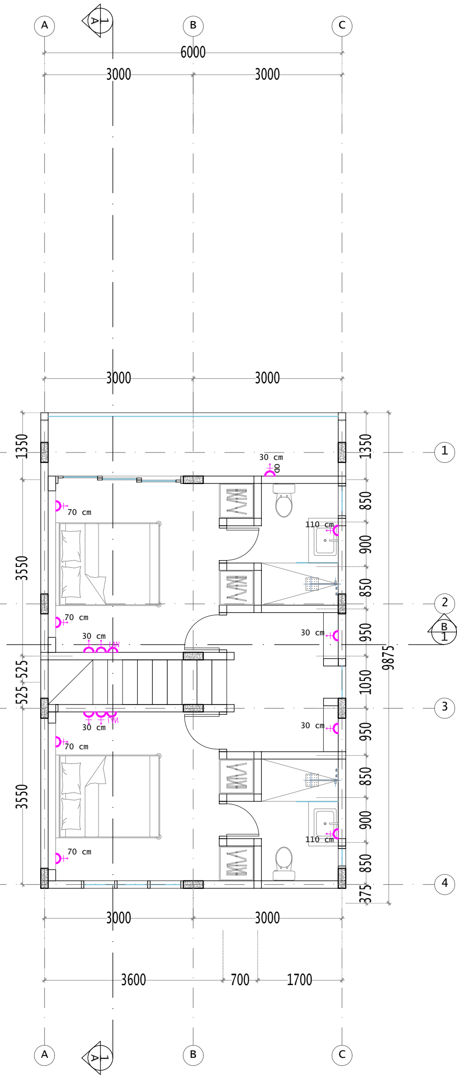
SECOND FLOOR SCALE 1 : 75
