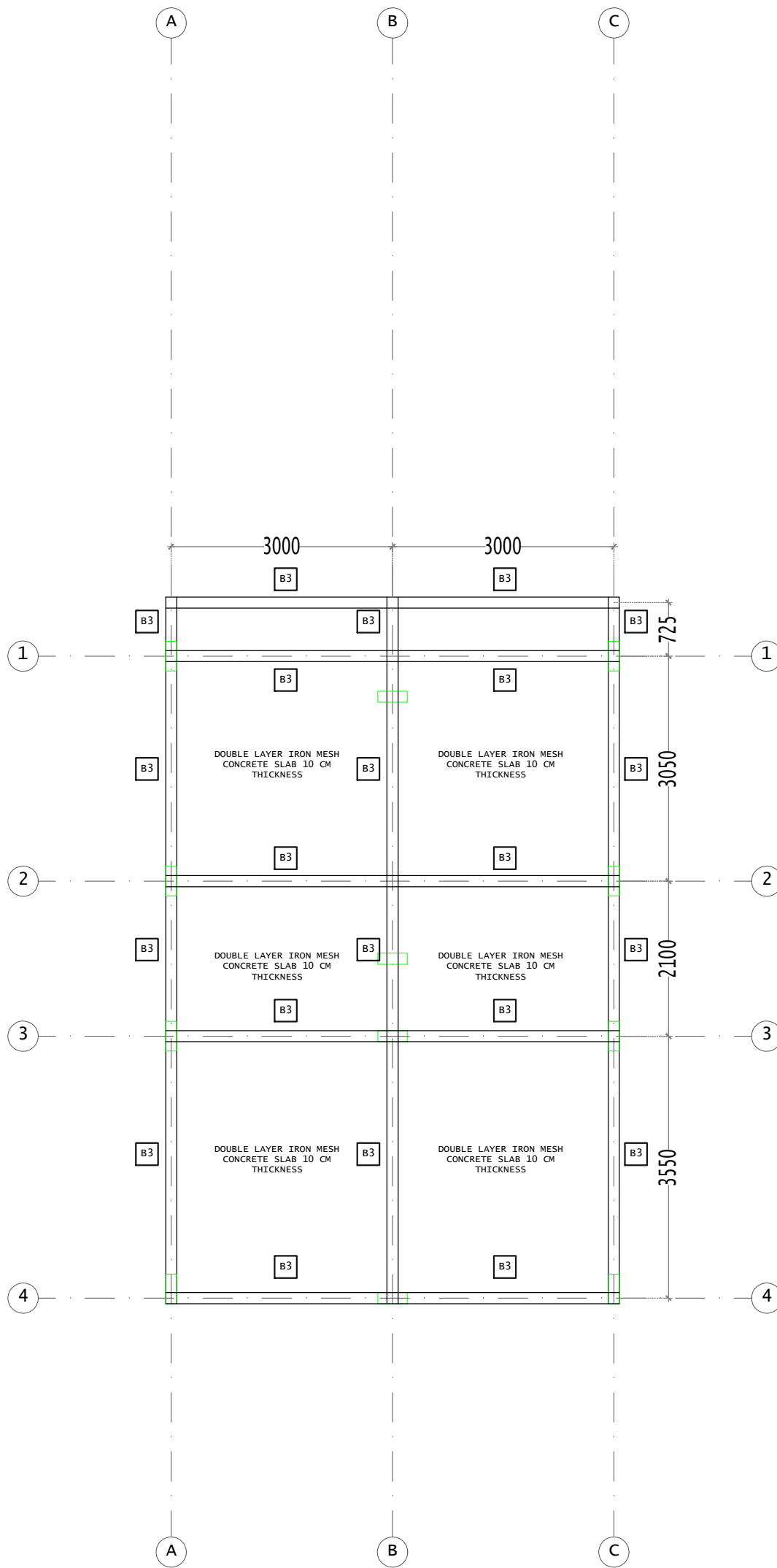
ROOF BEAM PLAN SCALE 1:75
