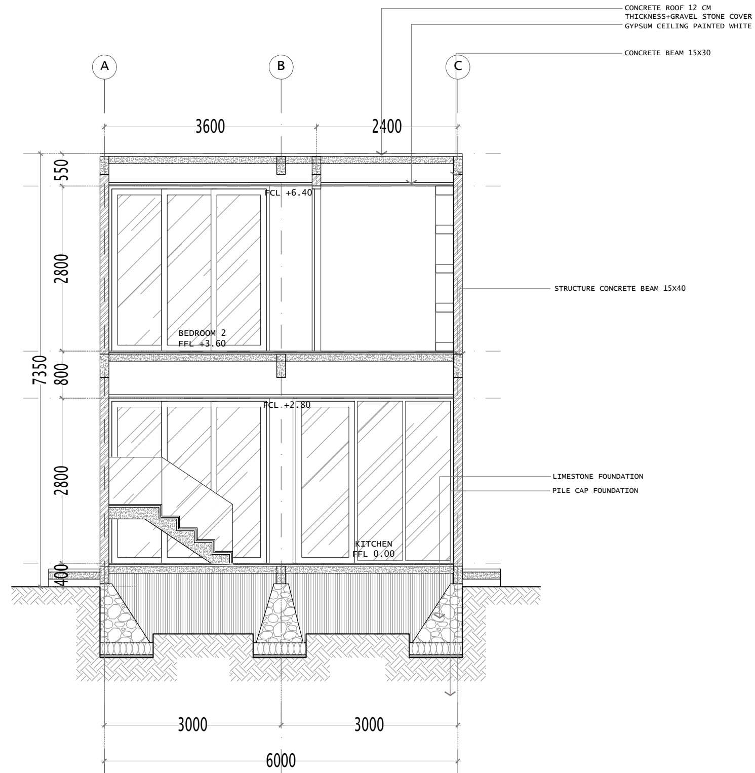
SECTION B-B SCALE 1:75
