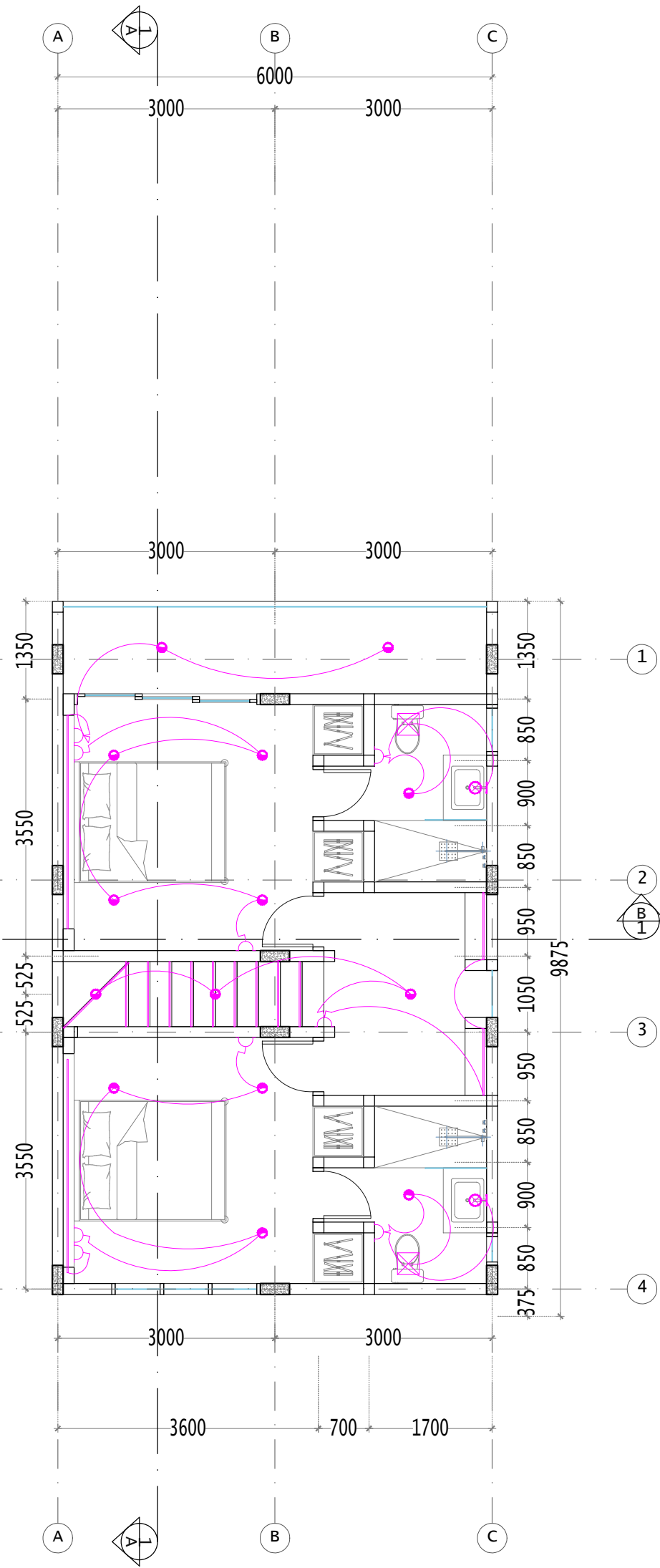
SECOND FLOOR LIGHTING PLAN | SCALE 1 : 75
