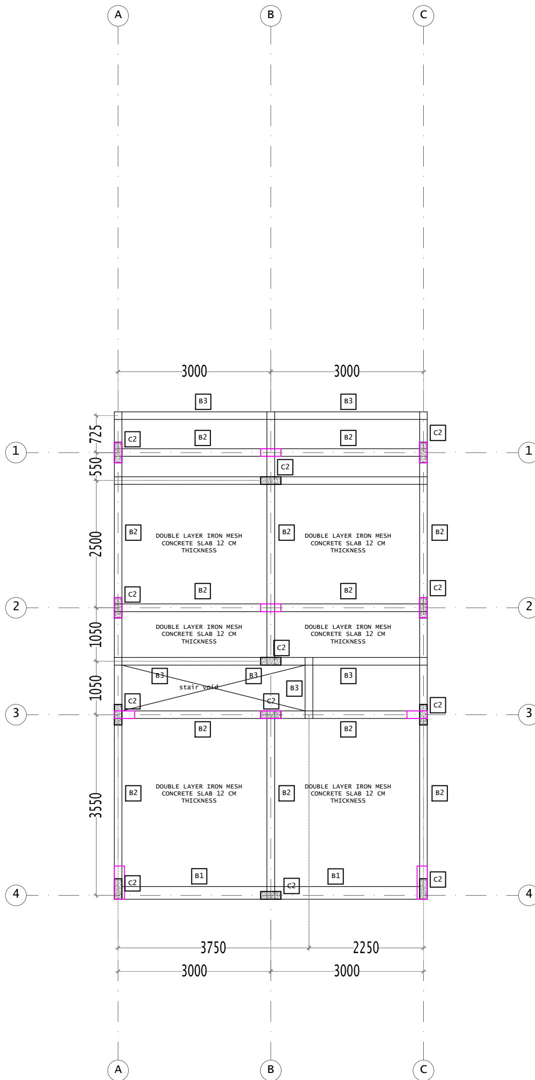
SECOND FLOOR BEAM PLAN SCALE 1:75
