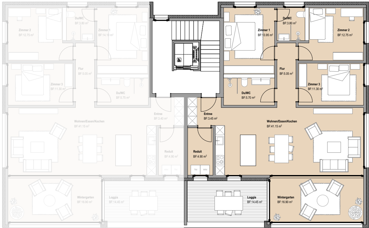
Whg 6 - 4.5 Zi BF:121.00 m 2
