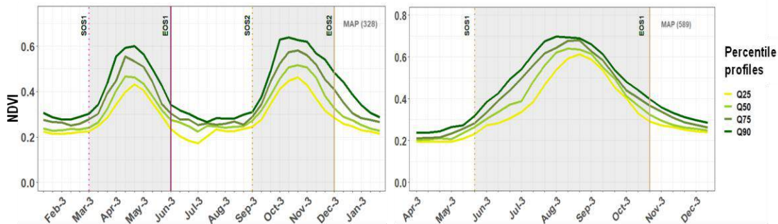
Figure 4: NVDI Profile
