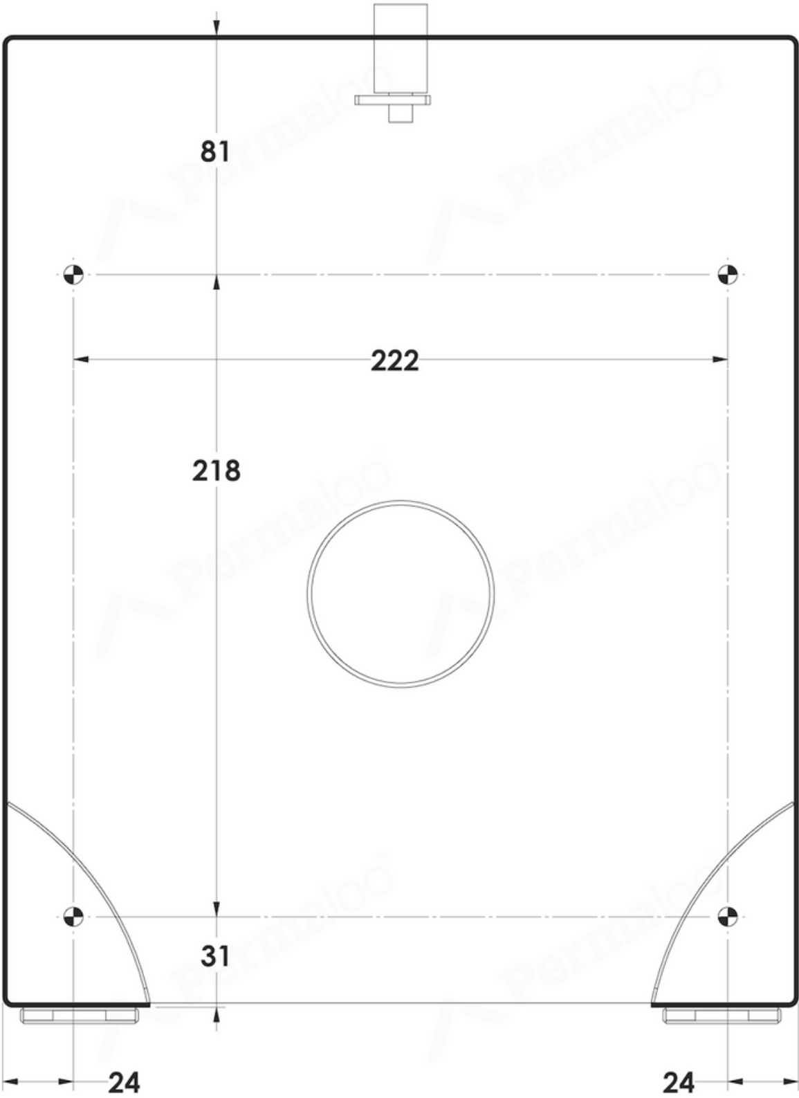
PERMA-001 SS Surface Mount Single Jumbo Roll Dispenser
