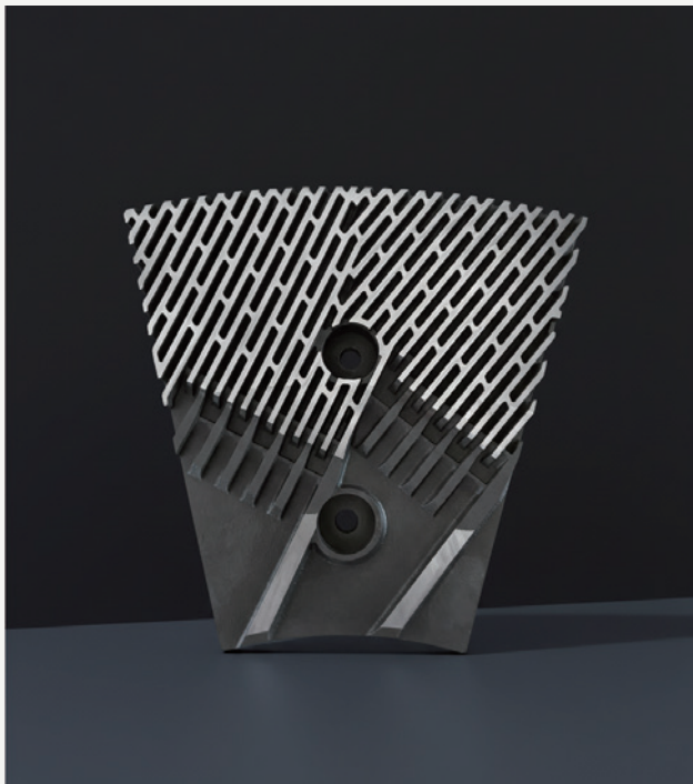
48" Segment compatible with Sufoma 48" defibrator
