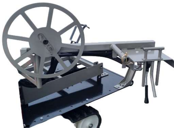
Hydraulic fire hose reel HS Part. 531 0148-98
