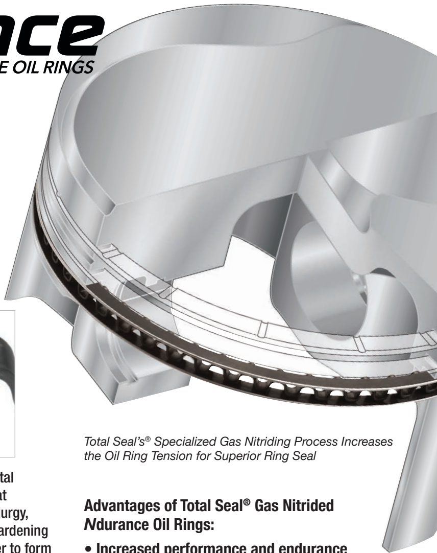
Nitride heat treating process transforms the metallurgy of the expander and changes the color from gold to black
